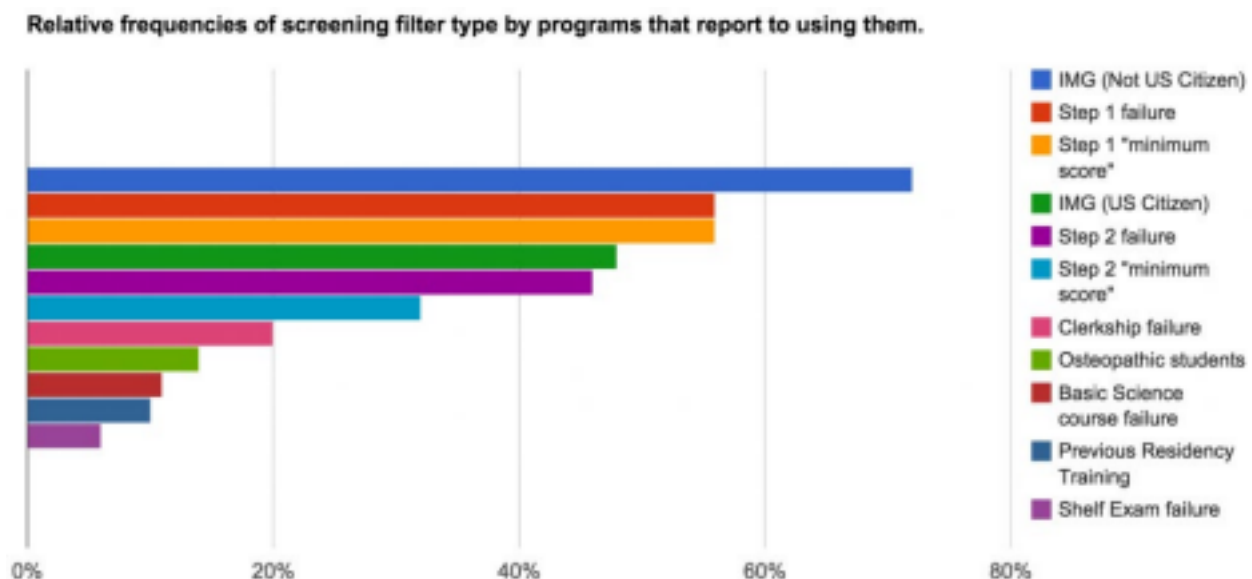
Figure 1. Relative frequencies of screening filter types by programs that report using them.
